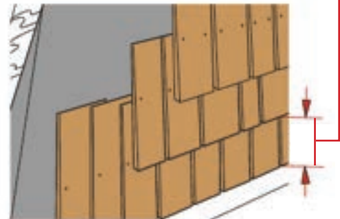
Sidewall Exposure
