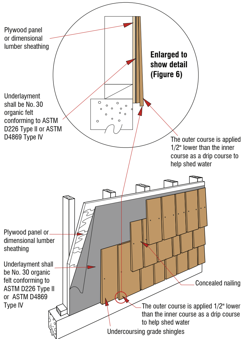
Figure 6: Single Coursing
