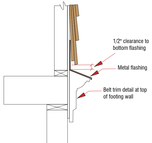
Figure 3b: Flashing
