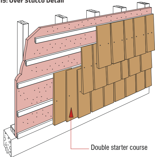
Figure 15: Over Stucco Detail
