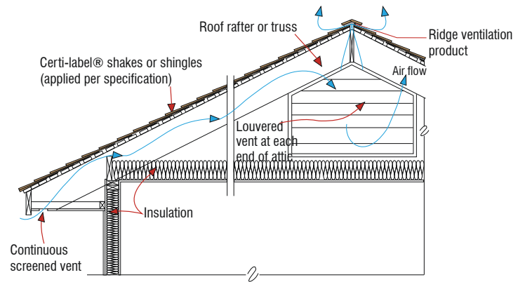
Figure 15a: Gable Roof With Attic
