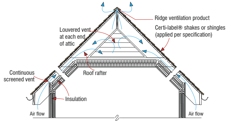
Figure 15b: Cathedral Ceiling With Partial Attic
