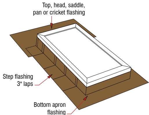
Figure 14a: Skylight Flashing
