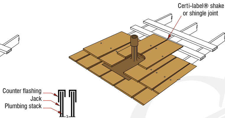
Figure 14e: Typical Projection Flashing
