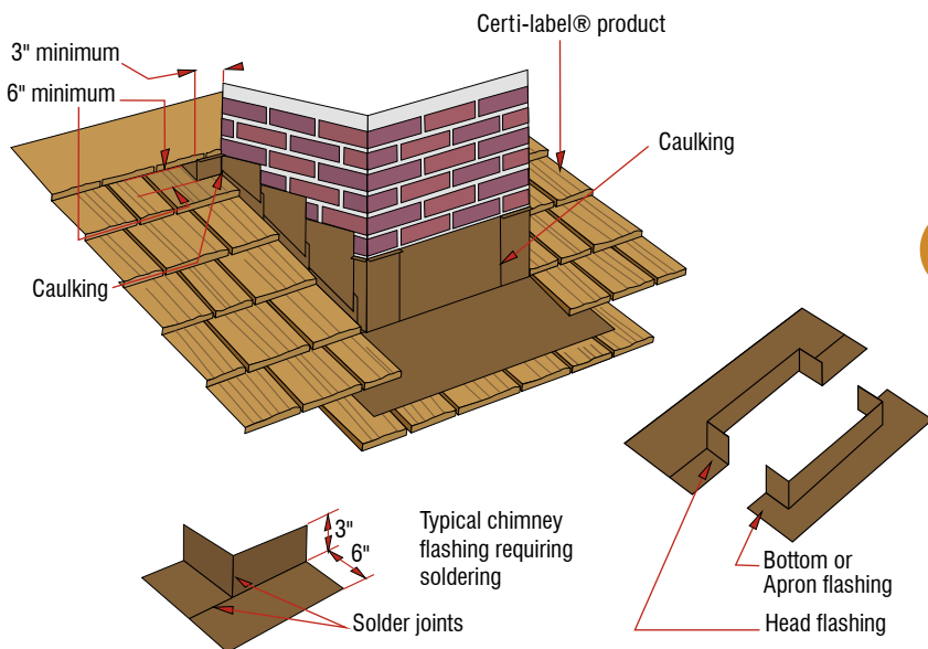
Figure 14c: Typical Projection Flashing
