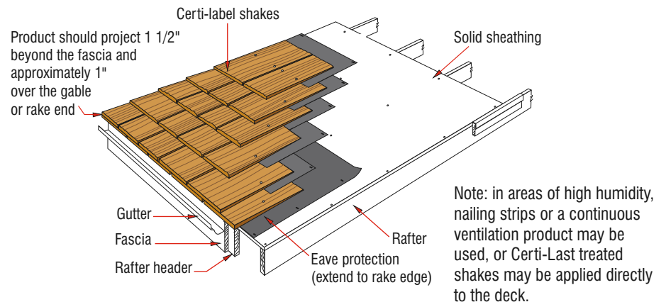
Figure 2: Solid Sheathing
