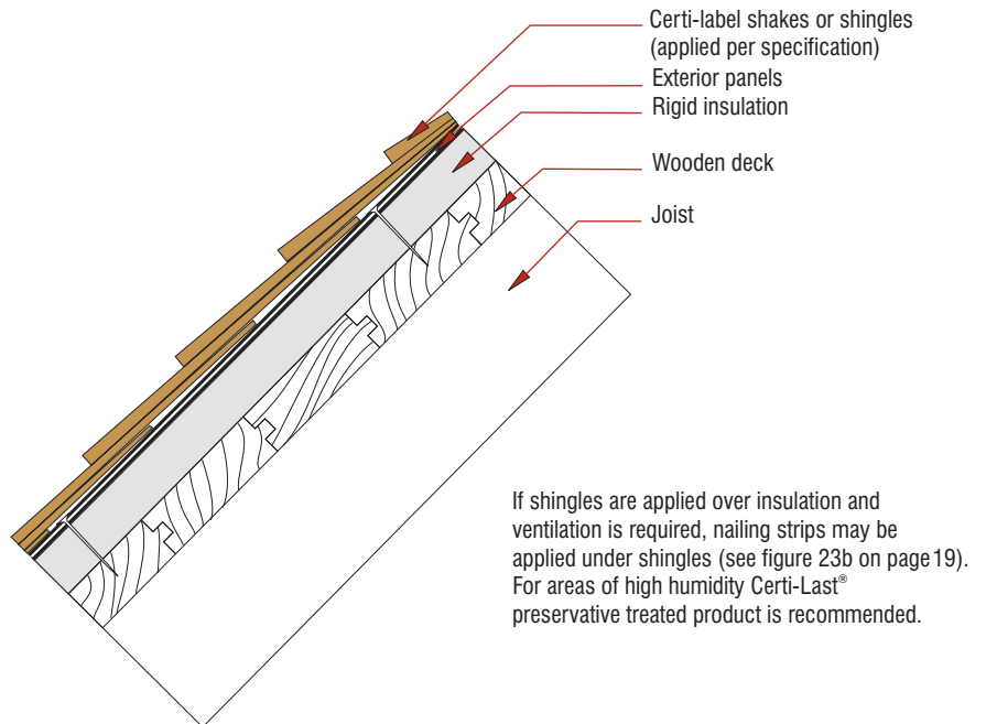
Figure 19: Specialty Roof Deck-Panels Over Insulation
