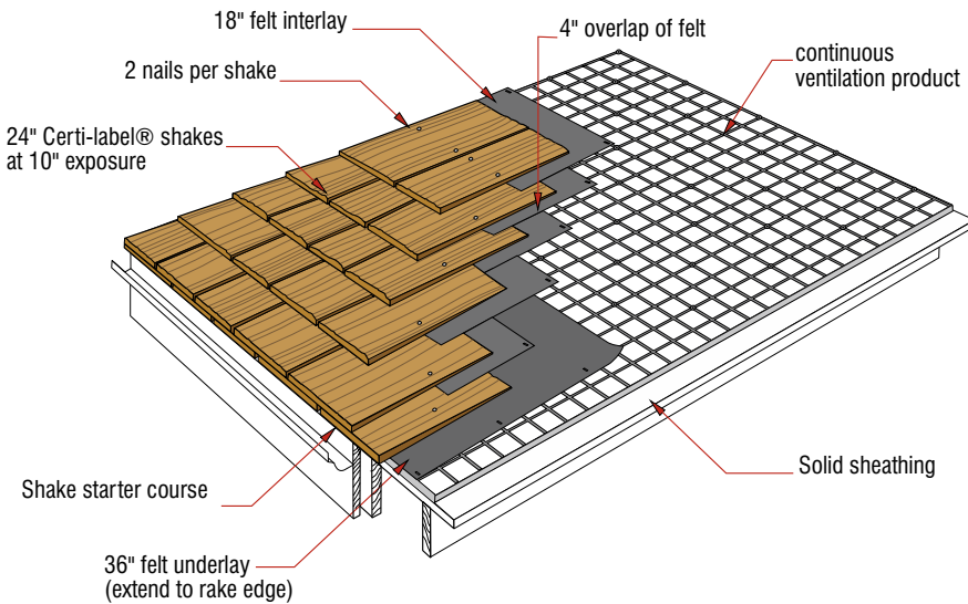
Figure 21d: Continuous Ventilation Product (rigid type)
