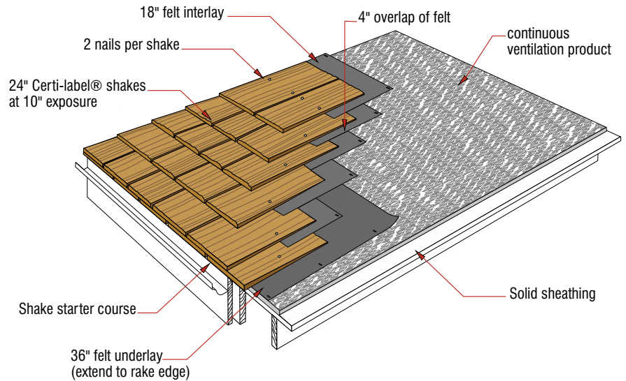
Figure 21c: Continuous Ventilation Product (mesh type)
