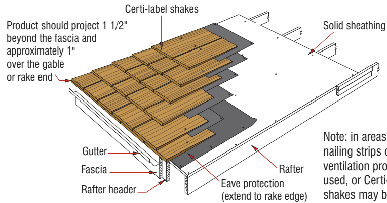
Figure 2: Solid Sheathing
