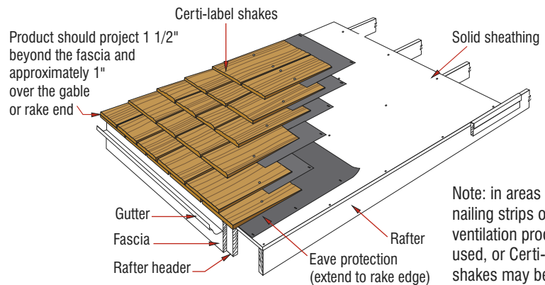
Figure 2: Solid Sheathing
