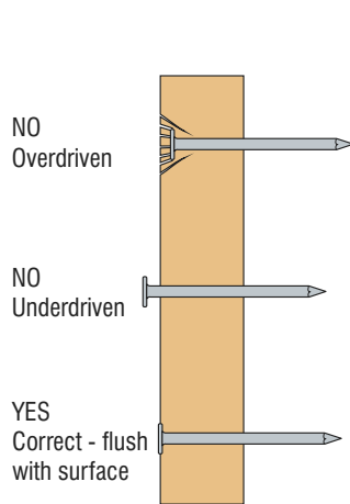
Figure 4: Nail Driving Detail
